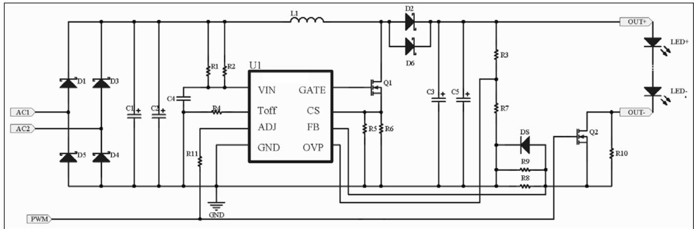
Figure 2: IS31LT3948 DEMO Board Schematic
