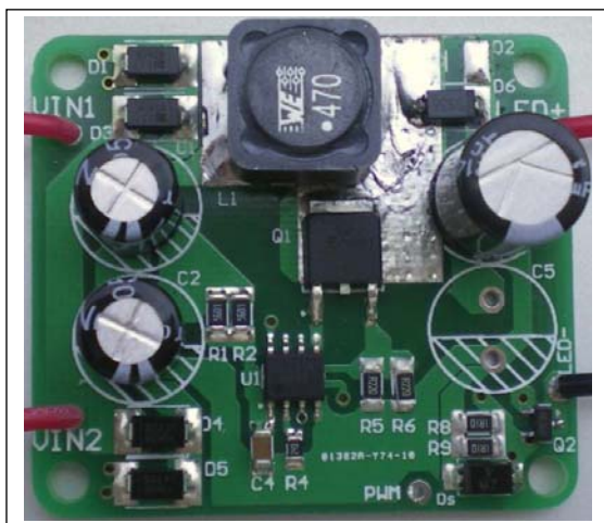
Figure 1: Photo of IS31LT3948 Evaluation Board
